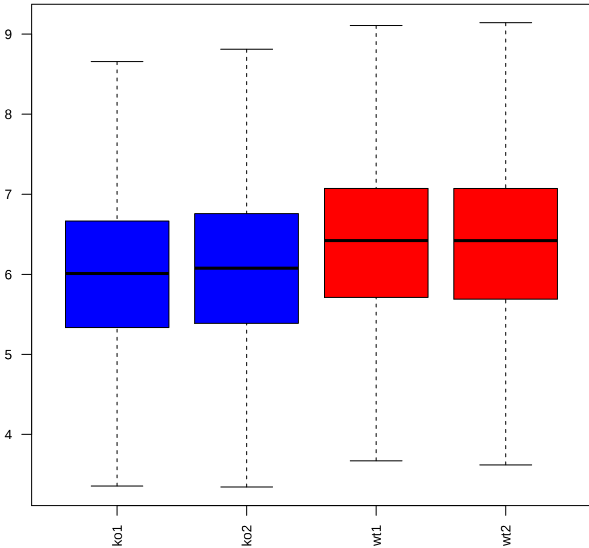
Boxplot
